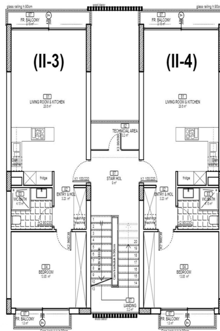
TYPE II FIRST FLOOR PLAN(1+1)
